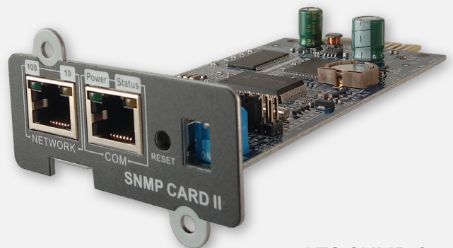
ATS SNMP Card Network Communication Interface
